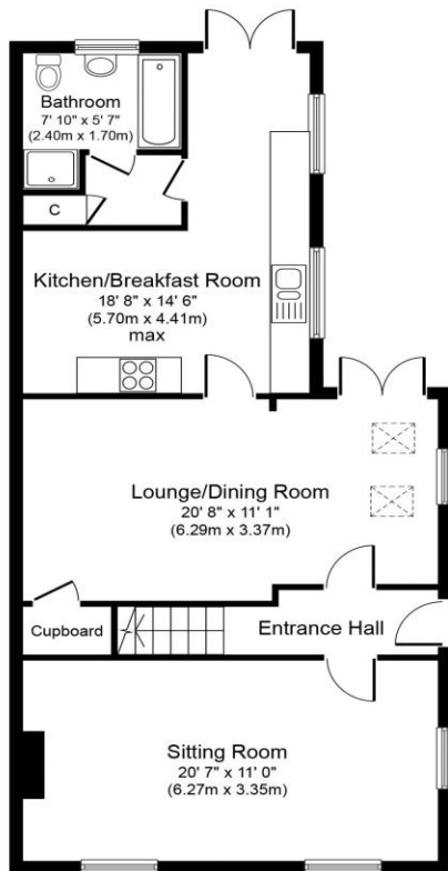
Ground Floor Approximate Floor Area 793 sq. ft. (73.7 sq. m.)
